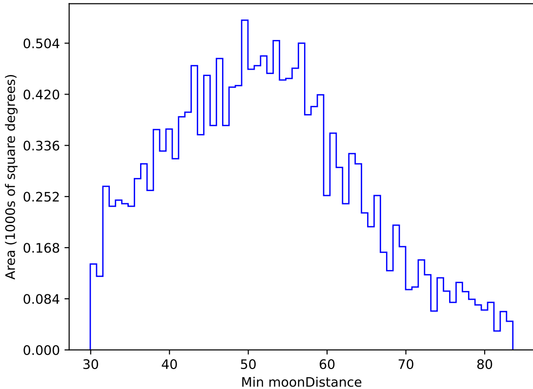
early_ss_template_fpextra2.0_v3.4_10yrs WFD u band: Min moonDistance
