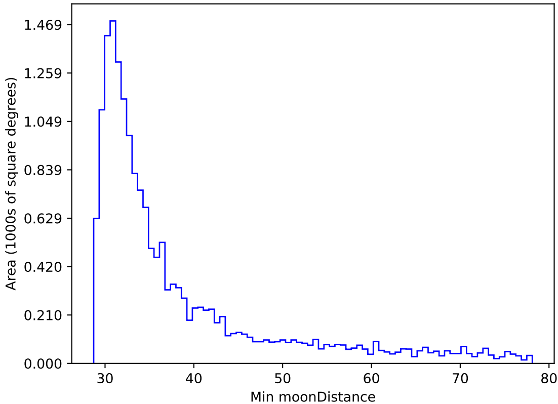
early_ss_template_fpextra2.0_v3.4_10yrs WFD r band: Min moonDistance
