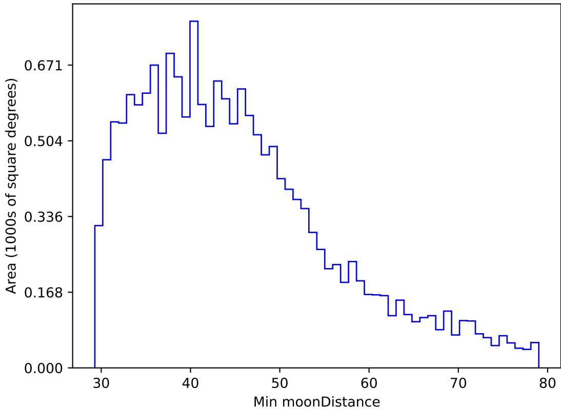
early_ss_template_fpextra2.0_v3.4_10yrs WFD g band: Min moonDistance
