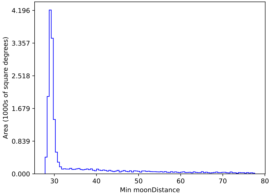
early_ss_template_fpextra2.0_v3.4_10yrs WFD all bands: Min moonDistance
