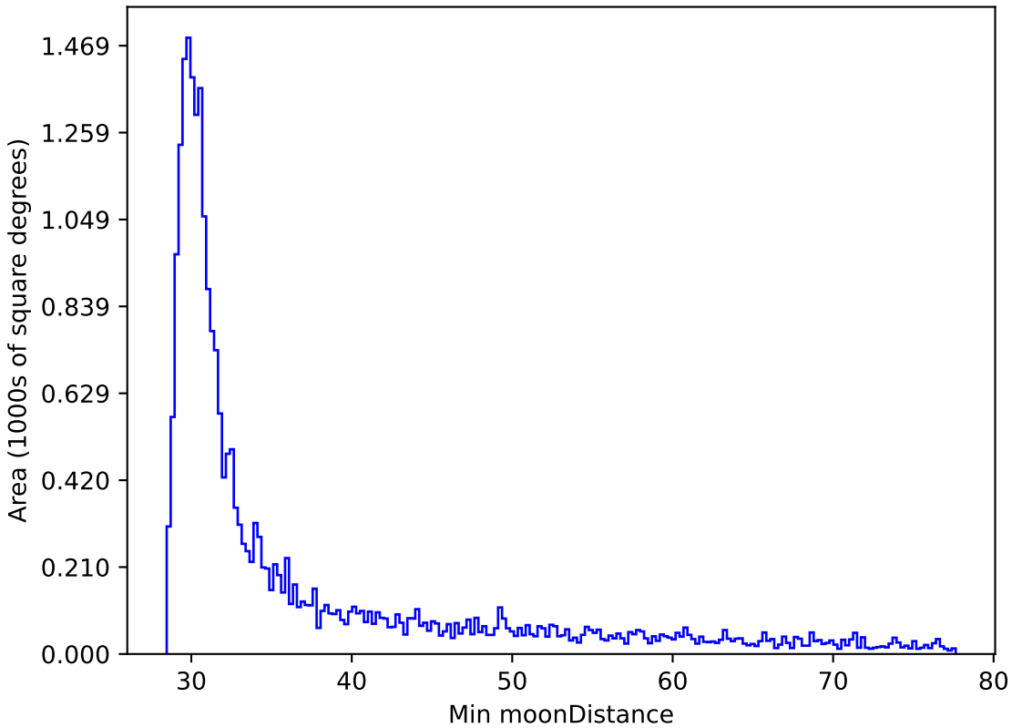
early_ss_template_fpextra2.0_v3.4_10yrs All sky i band: Min moonDistance
