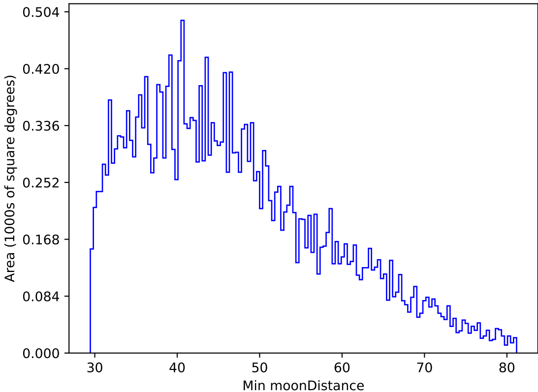
early_ss_template_fpextra2.0_v3.4_10yrs All sky g band: Min moonDistance
