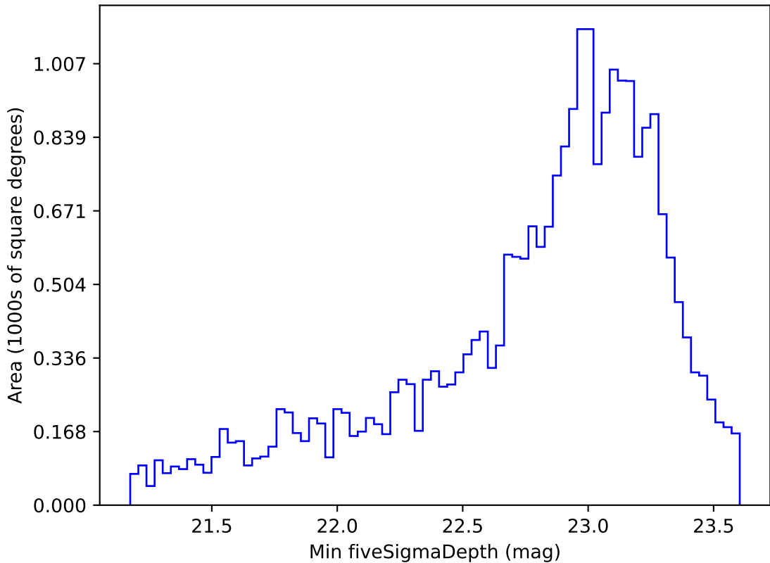
early_ss_template_fpextra2.0_v3.4_10yrs Yr 1 i band: Min fiveSigmaDepth
