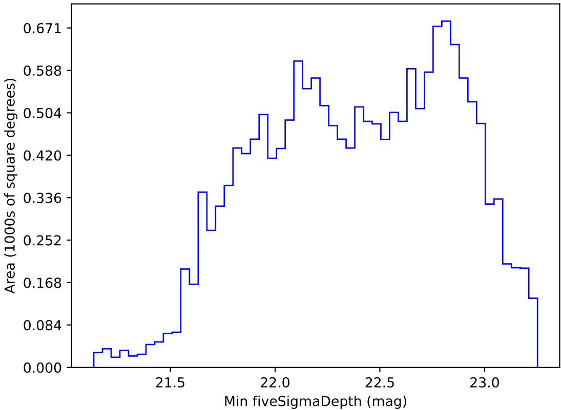
early_ss_template_fpextra2.0_v3.4_10yrs WFD r band: Min fiveSigmaDepth
