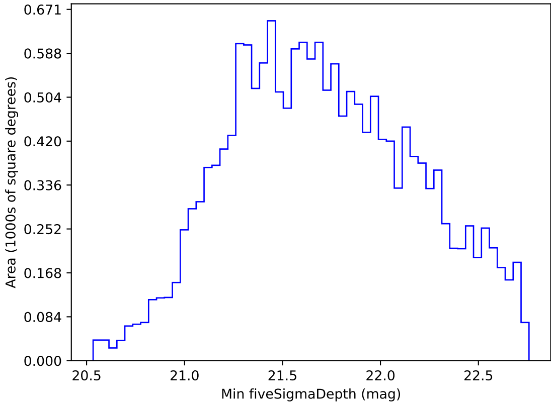
early_ss_template_fpextra2.0_v3.4_10yrs WFD i band: Min fiveSigmaDepth
