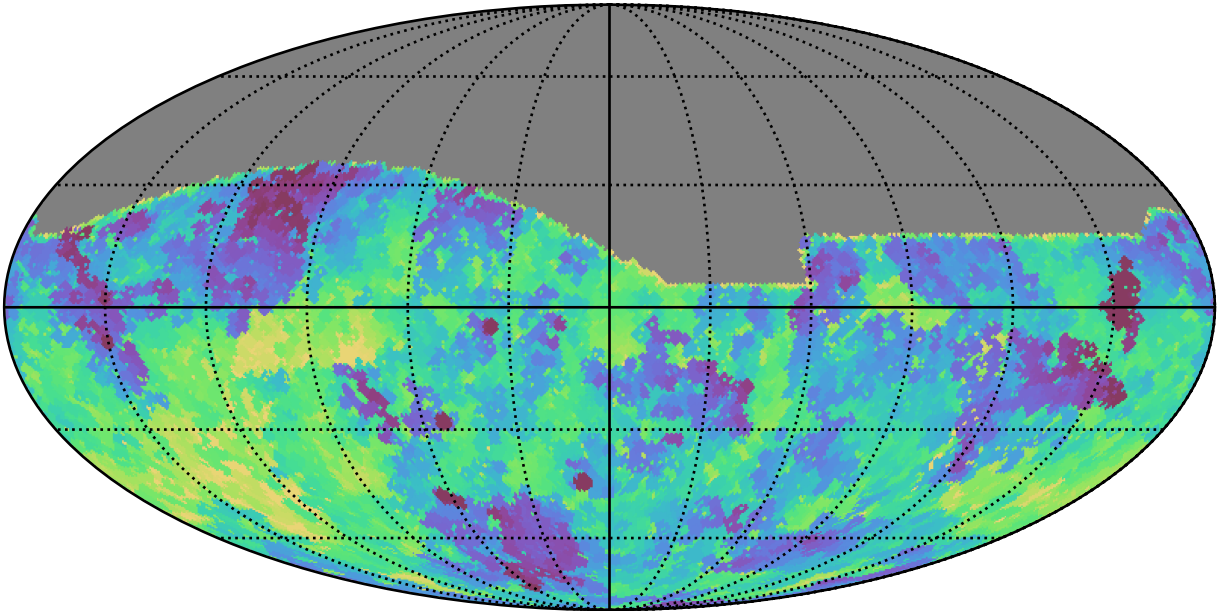
early_ss_template_fpextra2.0_v3.4_10yrs All sky g band: Min fiveSigmaDepth
