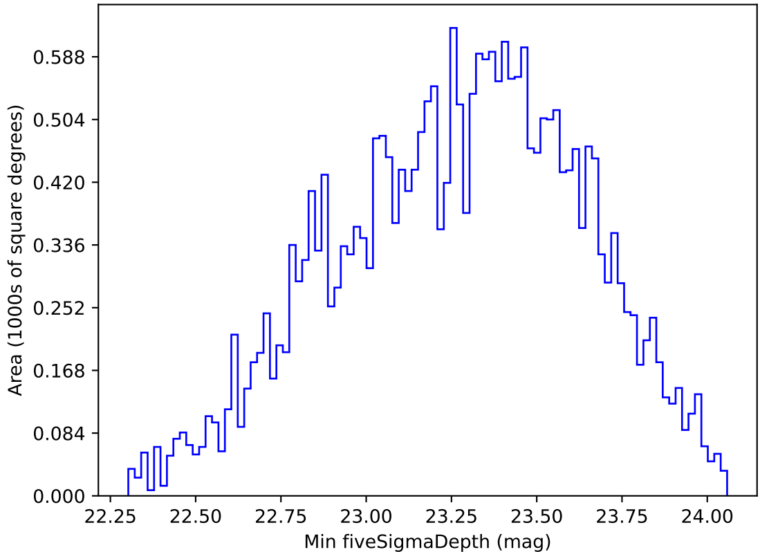
early_ss_template_fpextra2.0_v3.4_10yrs All sky g band: Min fiveSigmaDepth
