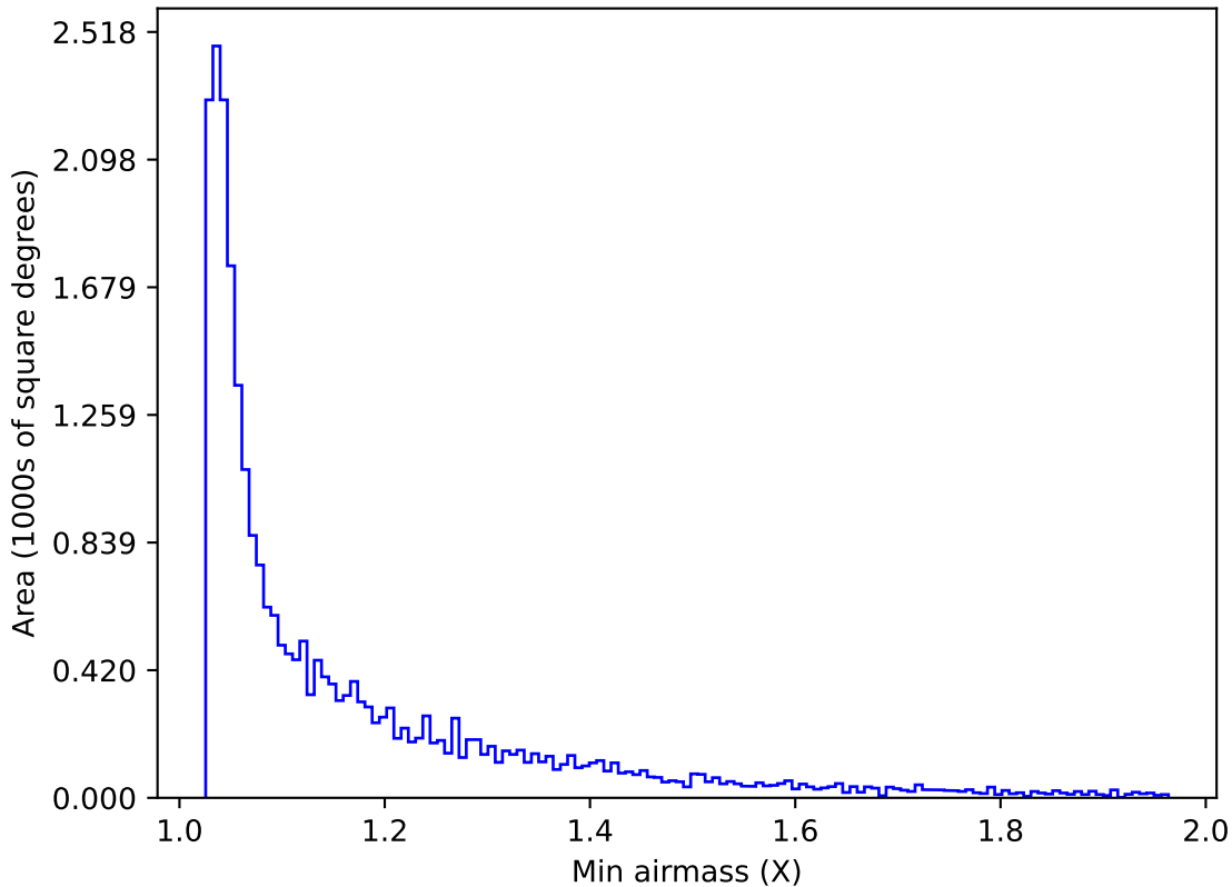
early_ss_template_fpextra2.0_v3.4_10yrs Yr 1 z band: Min airmass
