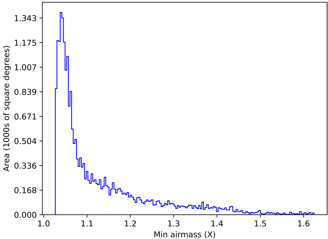
early_ss_template_fpextra2.0_v3.4_10yrs Yr 1 y band: Min airmass
