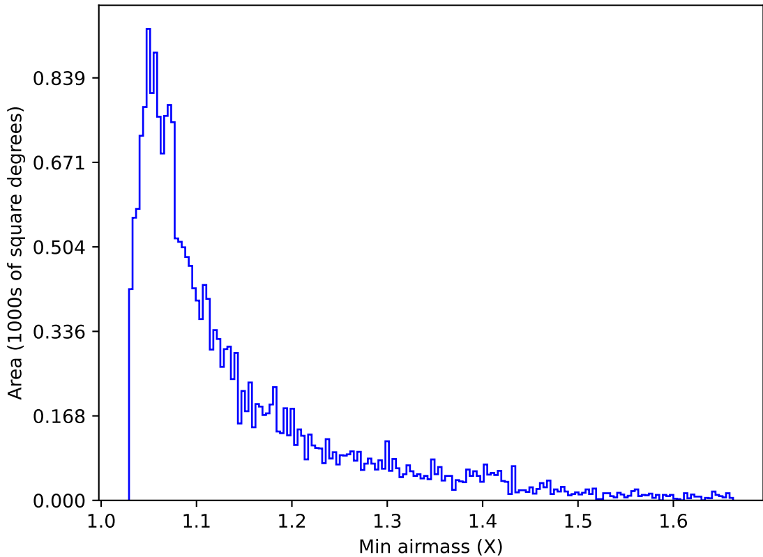
early_ss_template_fpextra2.0_v3.4_10yrs Yr 1 u band: Min airmass
