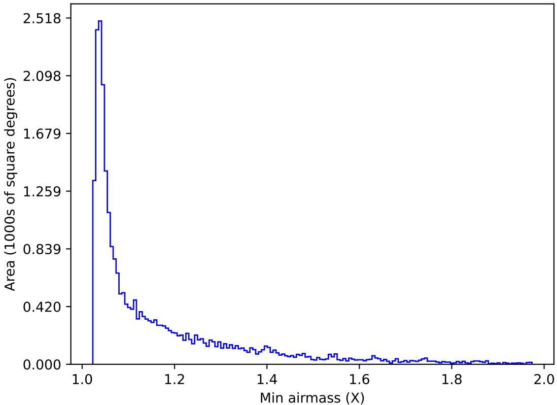
early_ss_template_fpextra2.0_v3.4_10yrs Yr 1 r band: Min airmass
