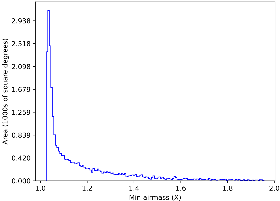
early_ss_template_fpextra2.0_v3.4_10yrs Yr 1 i band: Min airmass
