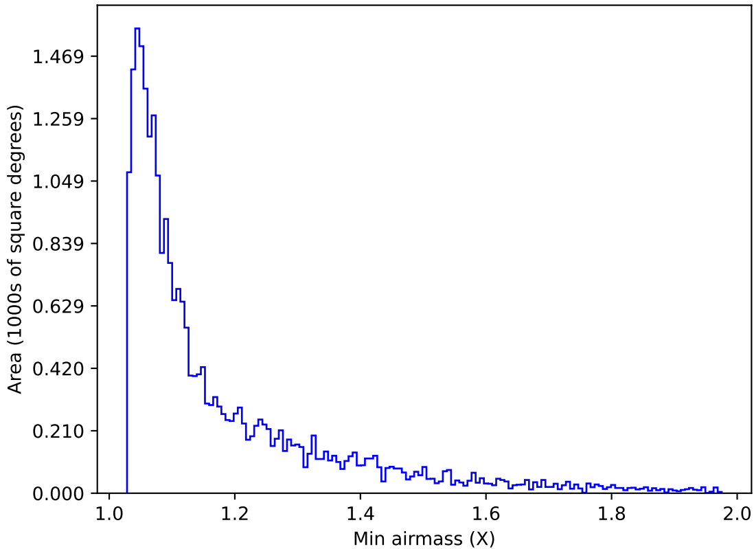
early_ss_template_fpextra2.0_v3.4_10yrs Yr 1 g band: Min airmass
