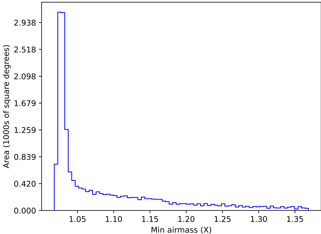
early_ss_template_fpextra2.0_v3.4_10yrs WFD z band: Min airmass
