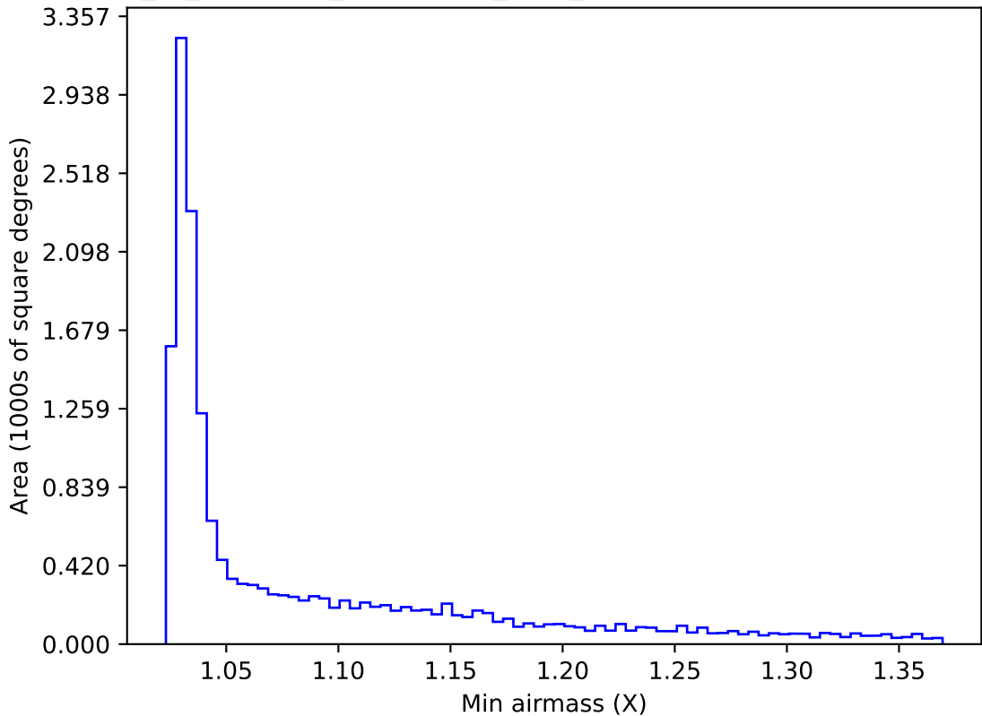
early_ss_template_fpextra2.0_v3.4_10yrs WFD y band: Min airmass
