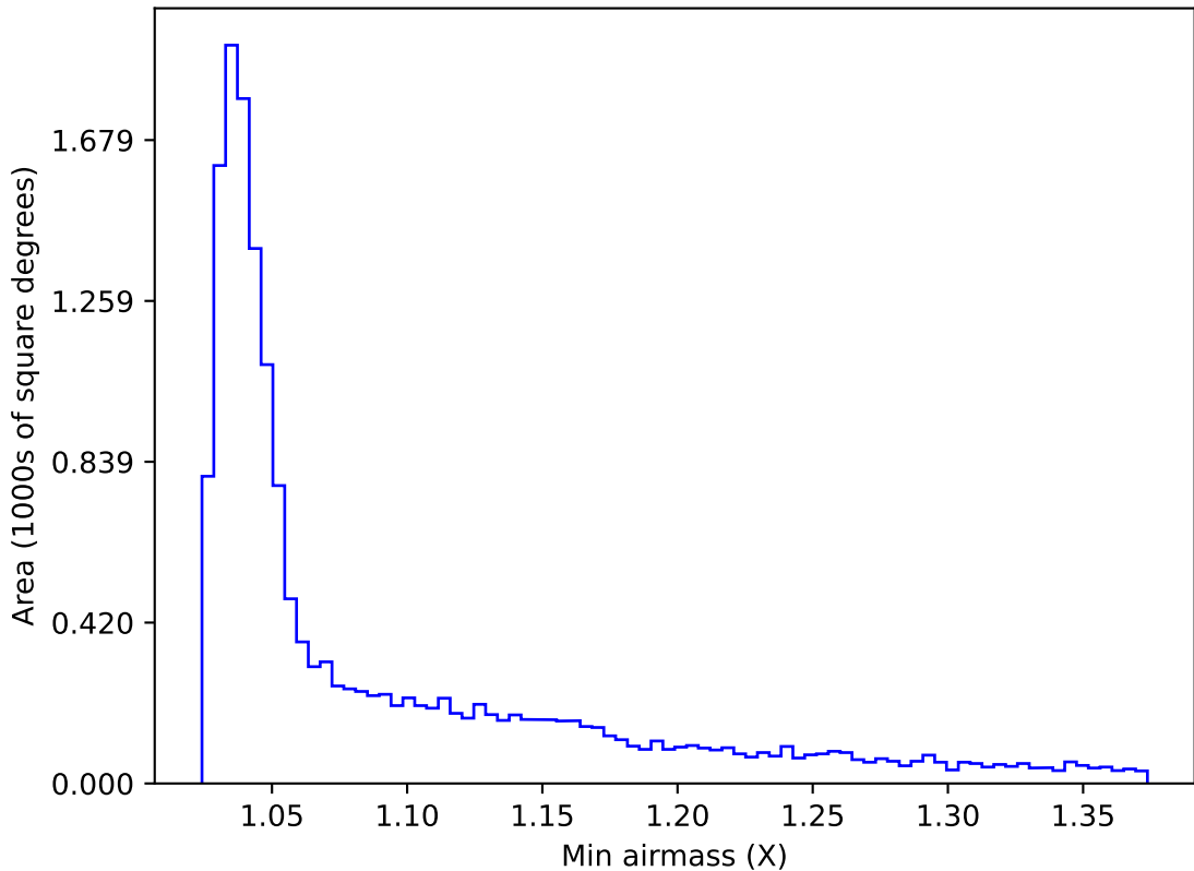
early_ss_template_fpextra2.0_v3.4_10yrs WFD u band: Min airmass
