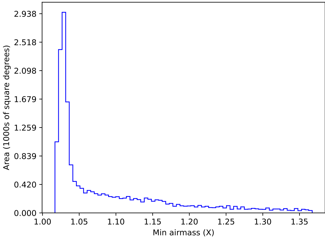
early_ss_template_fpextra2.0_v3.4_10yrs WFD r band: Min airmass
