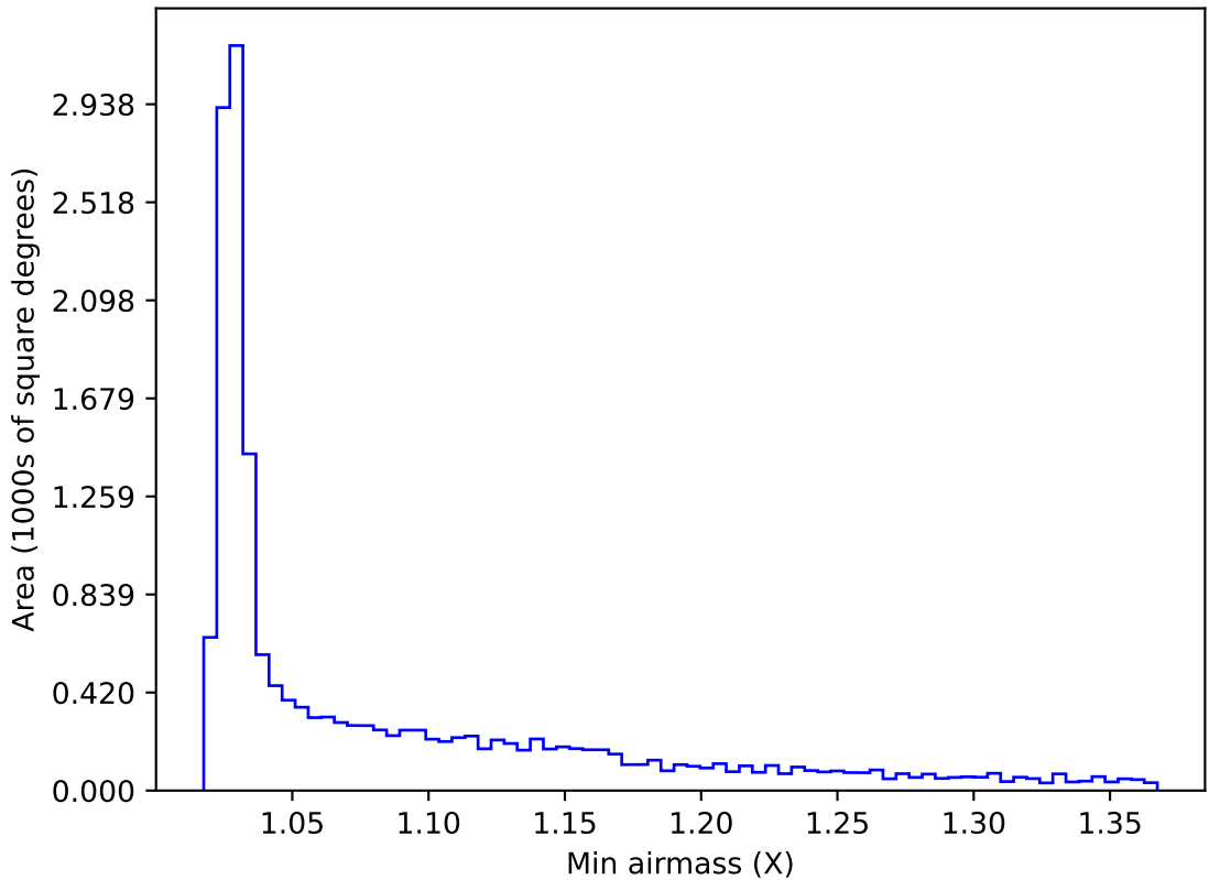
early_ss_template_fpextra2.0_v3.4_10yrs WFD i band: Min airmass
