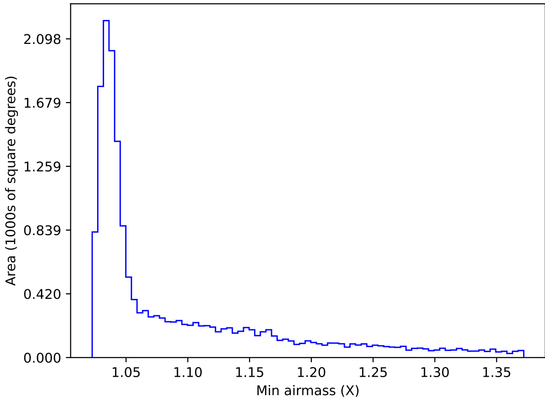
early_ss_template_fpextra2.0_v3.4_10yrs WFD g band: Min airmass
