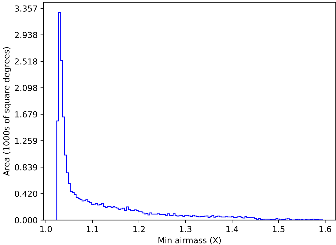
early_ss_template_fpextra2.0_v3.4_10yrs All sky y band: Min airmass
