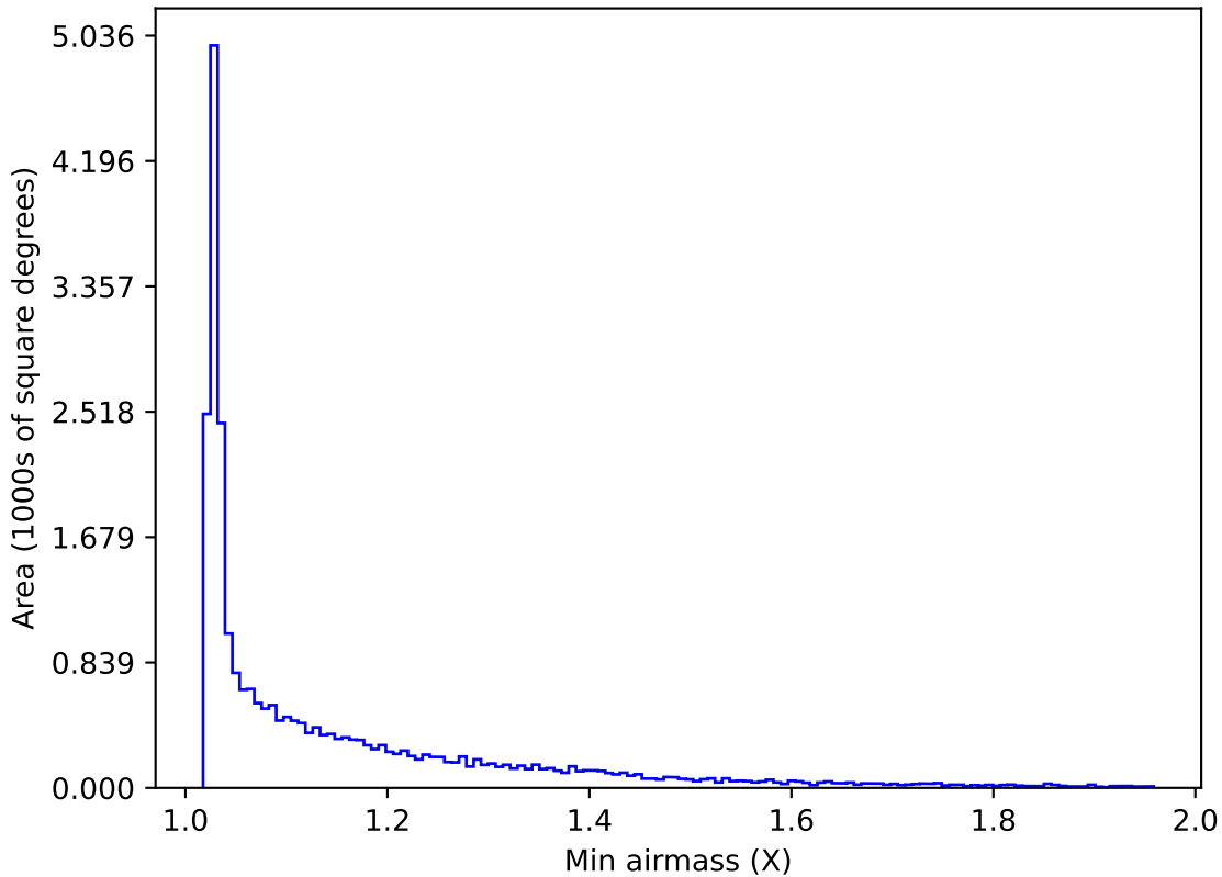
early_ss_template_fpextra2.0_v3.4_10yrs All sky r band: Min airmass
