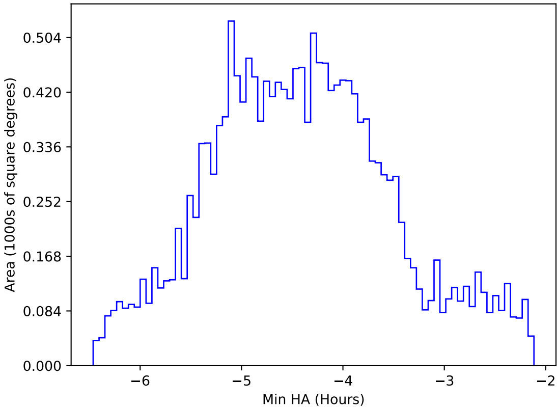
early_ss_template_fpextra2.0_v3.4_10yrs WFD z band: Min HA
