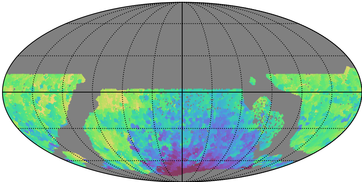
early_ss_template_fpextra2.0_v3.4_10yrs WFD y band: Min HA
