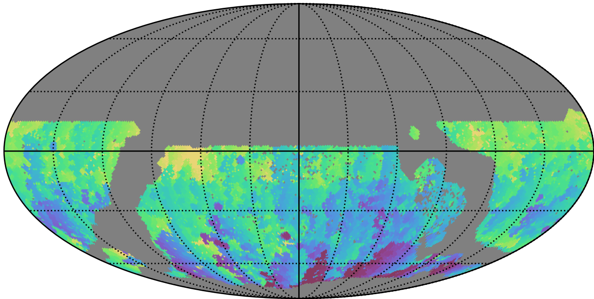
early_ss_template_fpextra2.0_v3.4_10yrs WFD u band: Min HA
