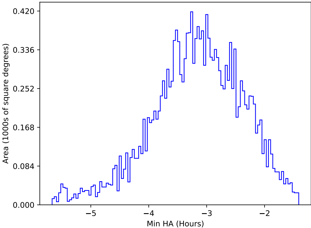
early_ss_template_fpextra2.0_v3.4_10yrs WFD u band: Min HA
