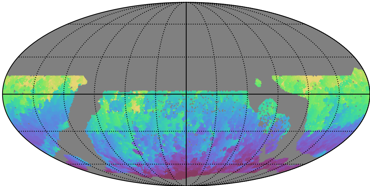
early_ss_template_fpextra2.0_v3.4_10yrs WFD i band: Min HA
