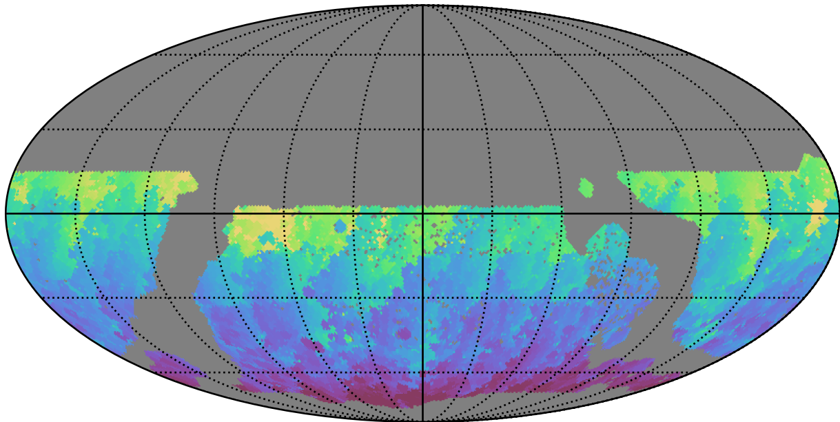
early_ss_template_fpextra2.0_v3.4_10yrs WFD g band: Min HA
