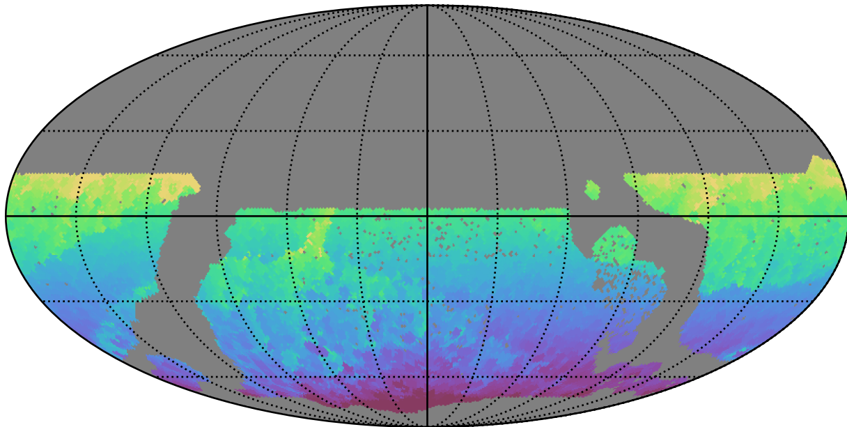
early_ss_template_fpextra2.0_v3.4_10yrs WFD all bands: Min HA
