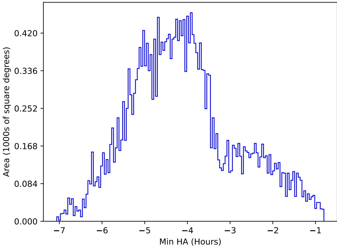
early_ss_template_fpextra2.0_v3.4_10yrs All sky z band: Min HA
