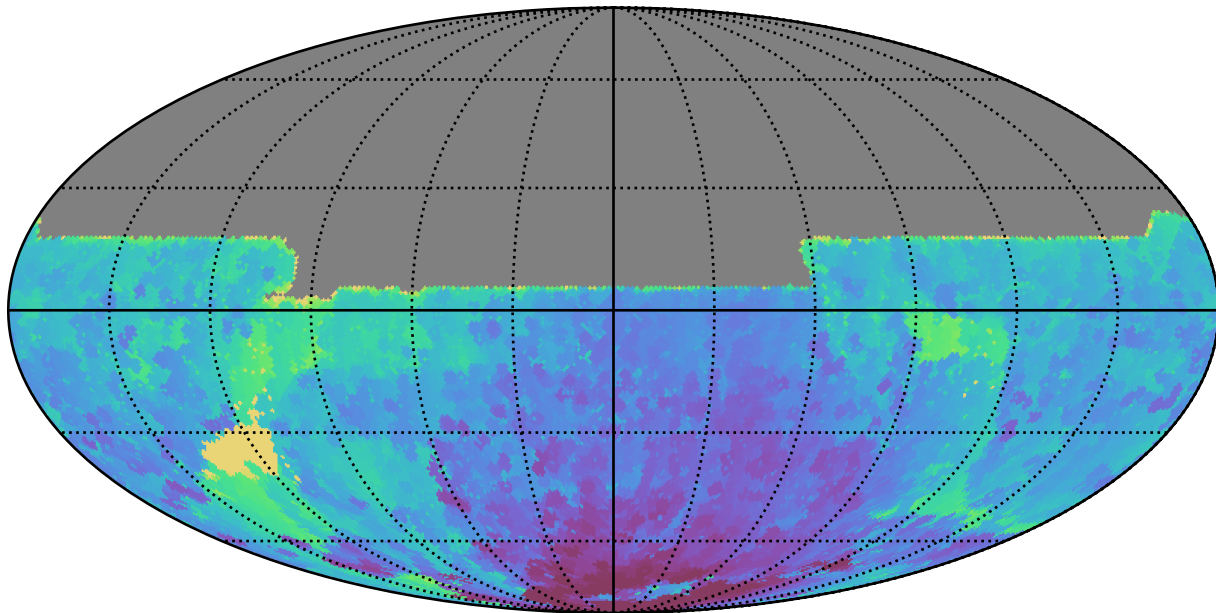
early_ss_template_fpextra2.0_v3.4_10yrs All sky y band: Min HA
