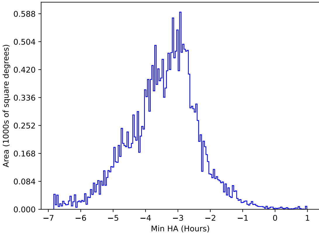
early_ss_template_fpextra2.0_v3.4_10yrs All sky y band: Min HA
