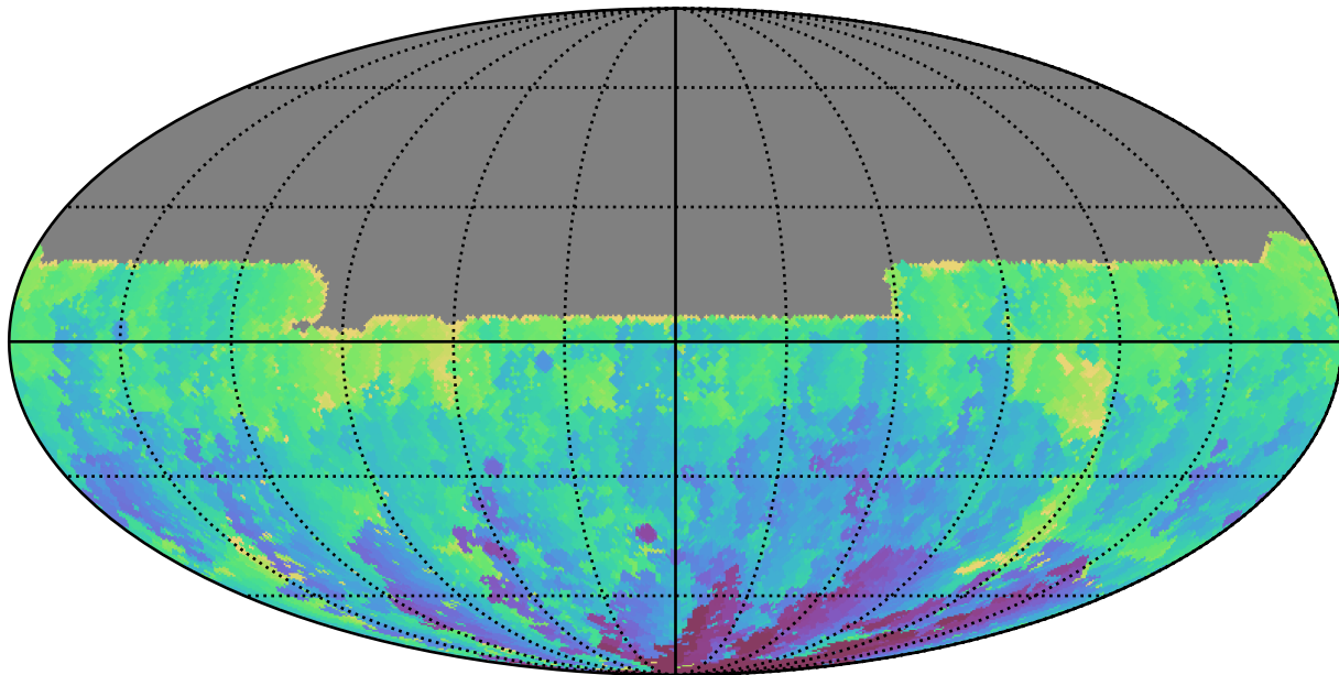
early_ss_template_fpextra2.0_v3.4_10yrs All sky u band: Min HA
