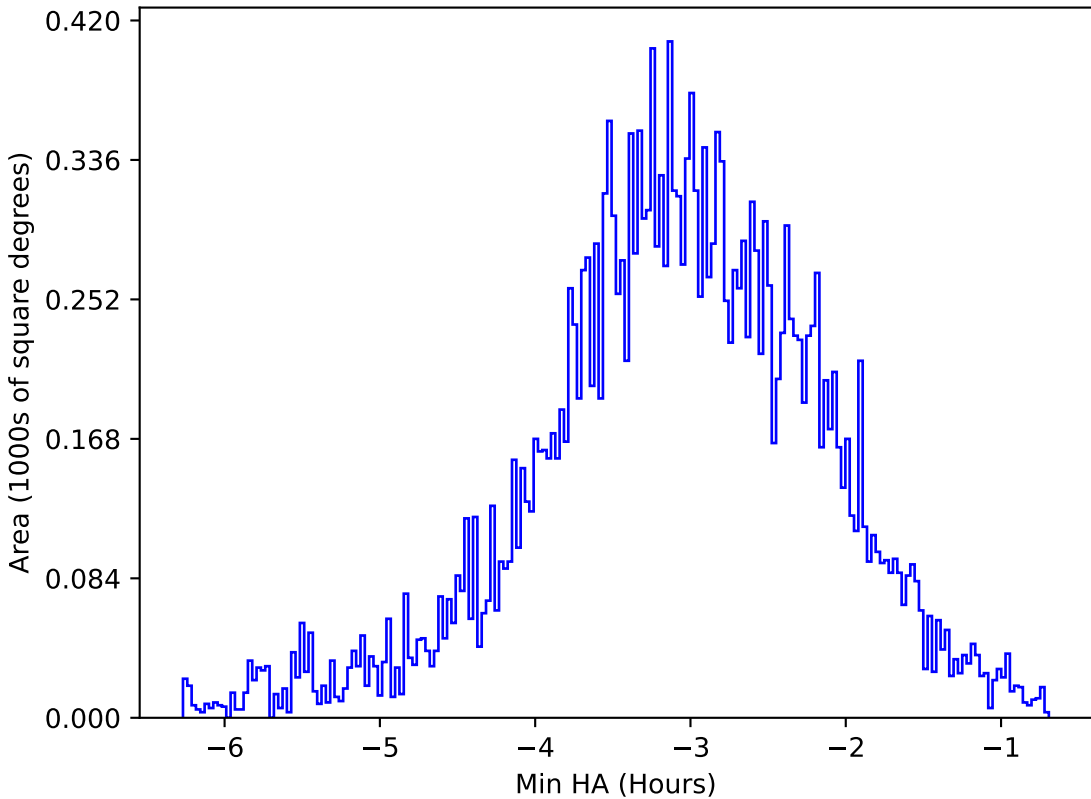
early_ss_template_fpextra2.0_v3.4_10yrs All sky u band: Min HA
