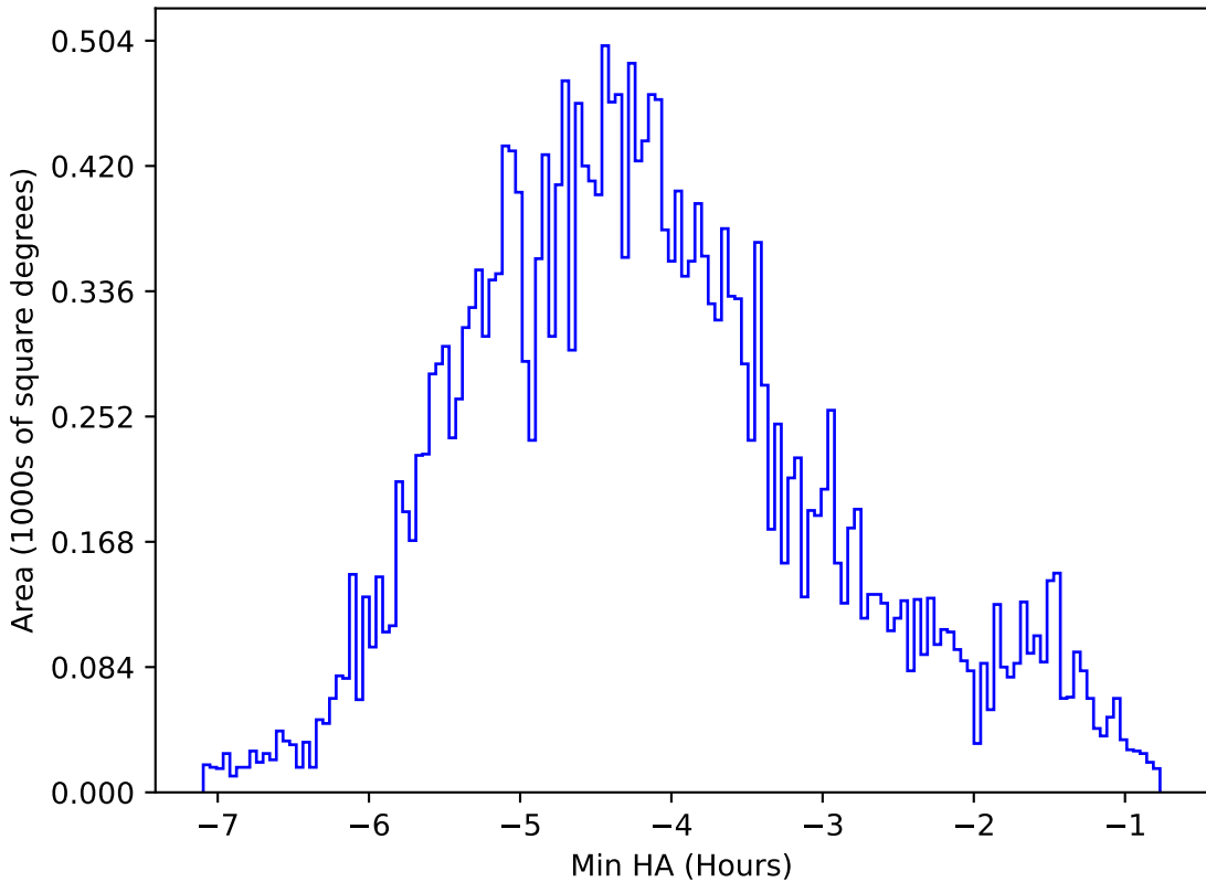
early_ss_template_fpextra2.0_v3.4_10yrs All sky r band: Min HA
