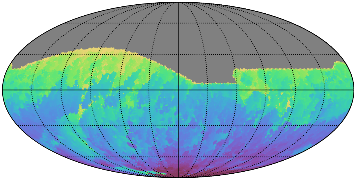
early_ss_template_fpextra2.0_v3.4_10yrs All sky i band: Min HA
