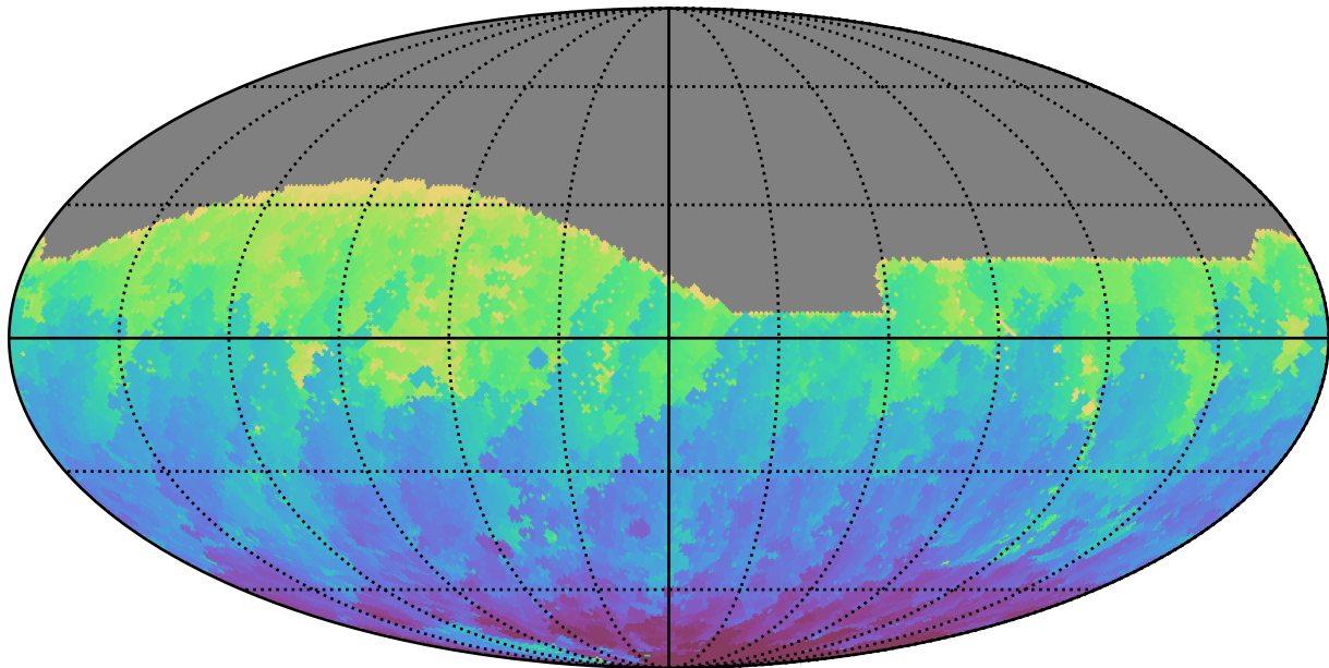
early_ss_template_fpextra2.0_v3.4_10yrs All sky g band: Min HA
