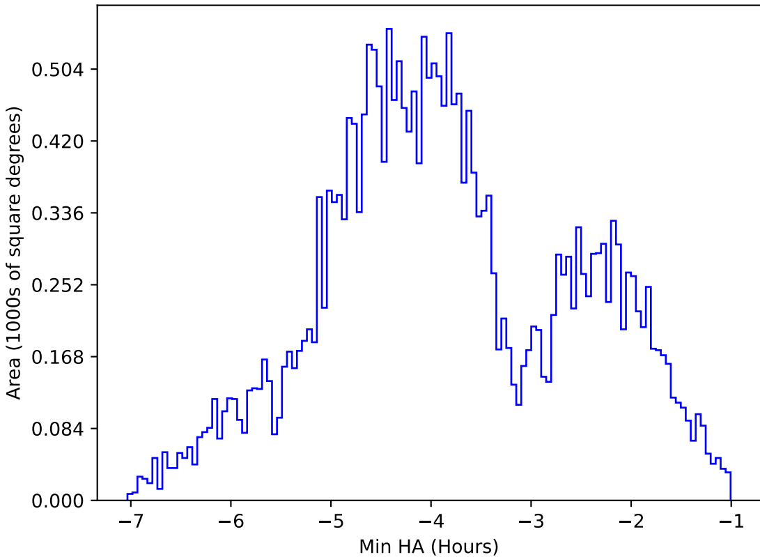
early_ss_template_fpextra2.0_v3.4_10yrs All sky g band: Min HA
