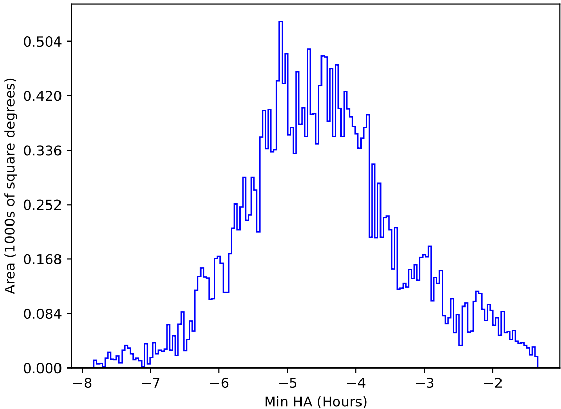
early_ss_template_fpextra2.0_v3.4_10yrs All sky all bands: Min HA
