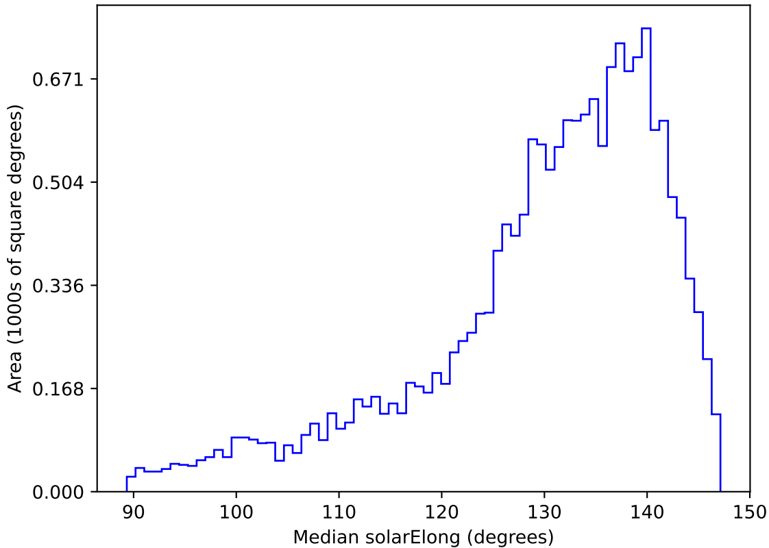
early_ss_template_fpextra2.0_v3.4_10yrs WFD y band: Median solarElong
