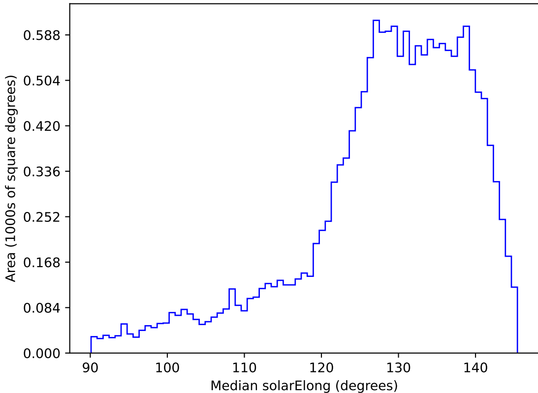
early_ss_template_fpextra2.0_v3.4_10yrs WFD i band: Median solarElong
