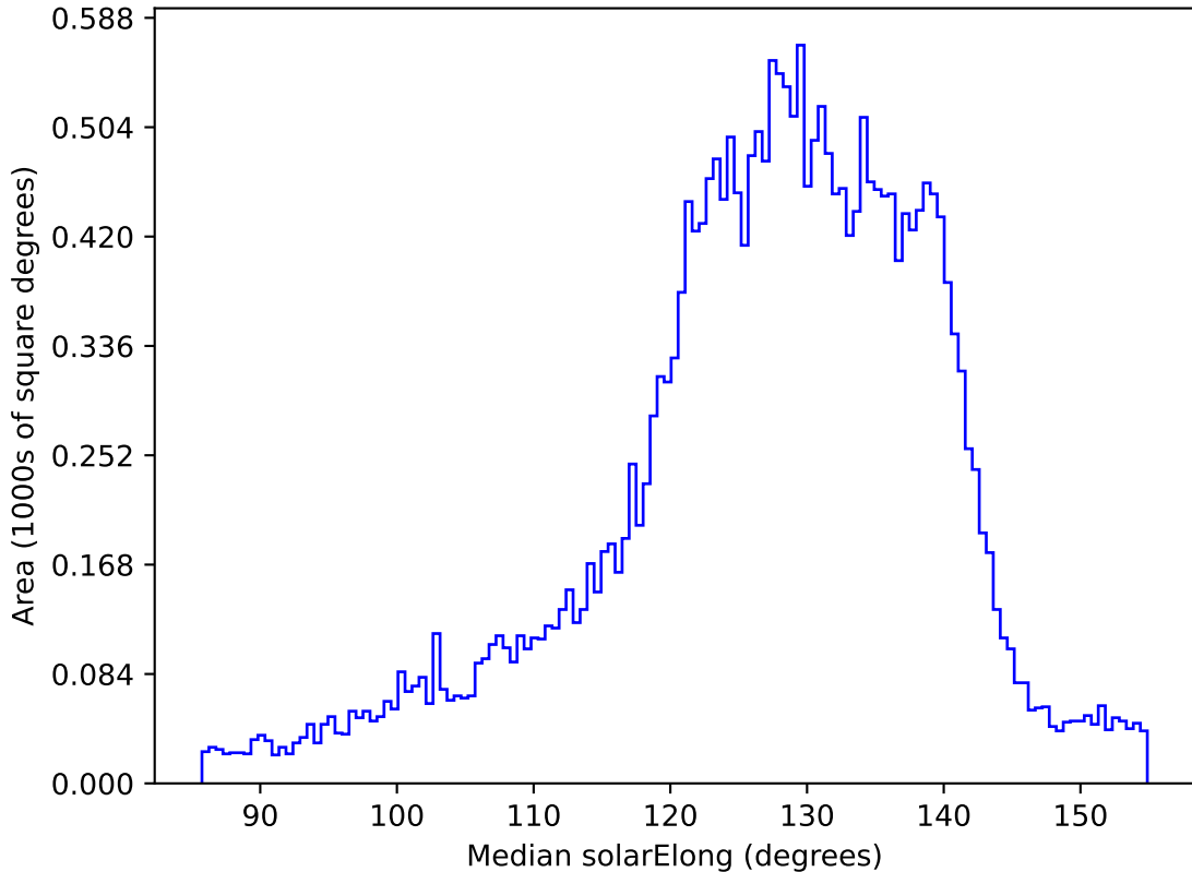
early_ss_template_fpextra2.0_v3.4_10yrs All sky z band: Median solarElong
