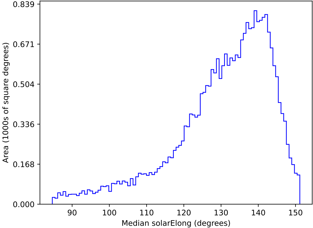
early_ss_template_fpextra2.0_v3.4_10yrs All sky r band: Median solarElong
