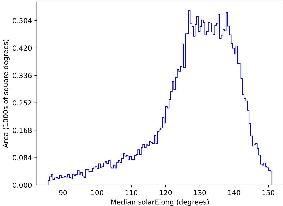
early_ss_template_fpextra2.0_v3.4_10yrs All sky i band: Median solarElong
