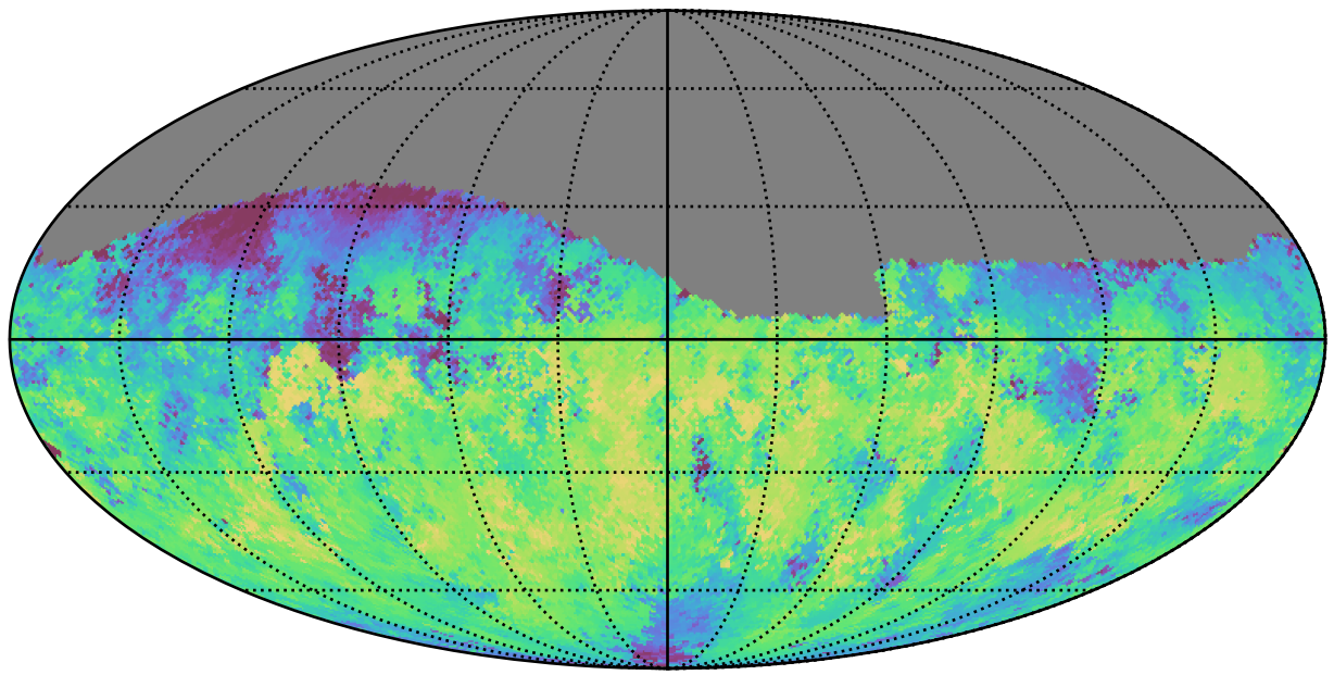
early_ss_template_fpextra2.0_v3.4_10yrs Yr 1 z band: Median skyBrightness
