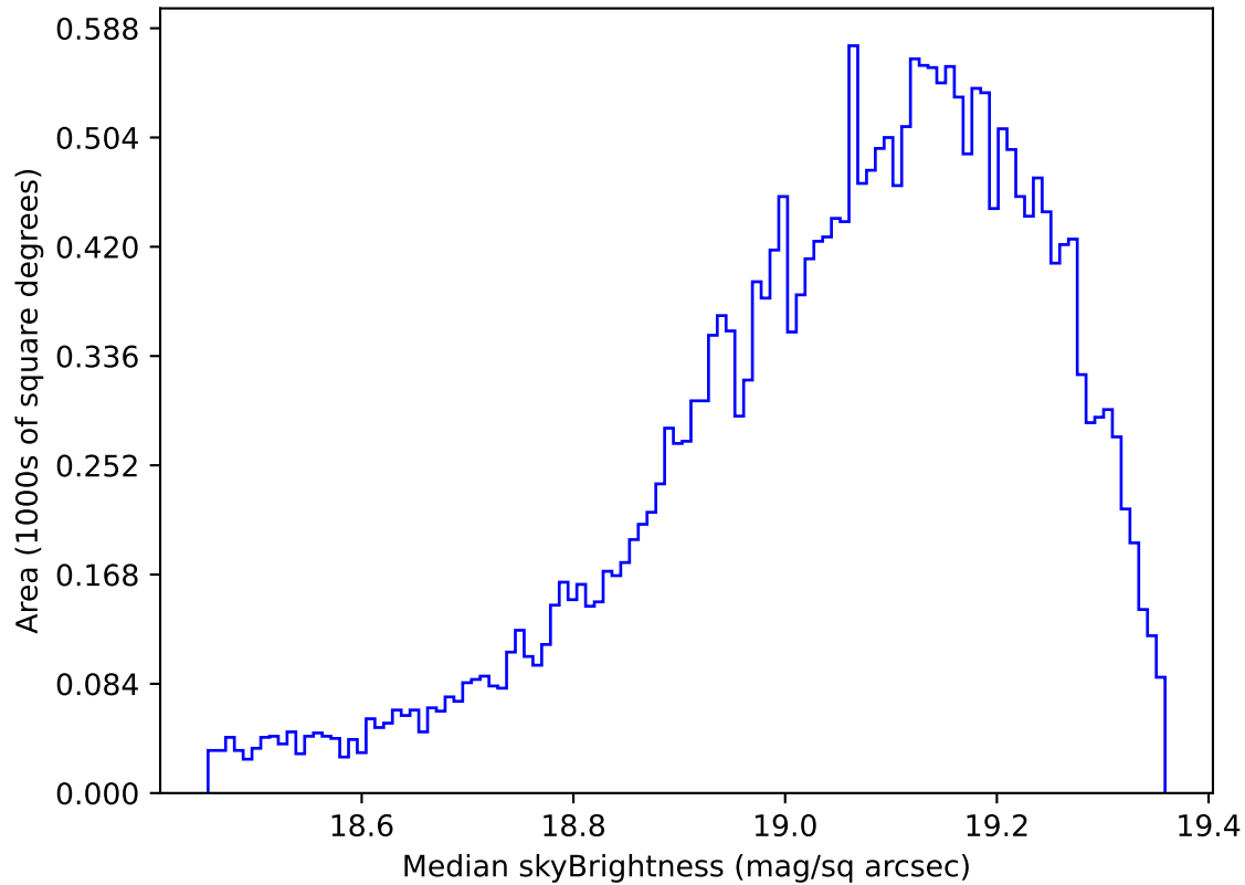
early_ss_template_fpextra2.0_v3.4_10yrs Yr 1 z band: Median skyBrightness
