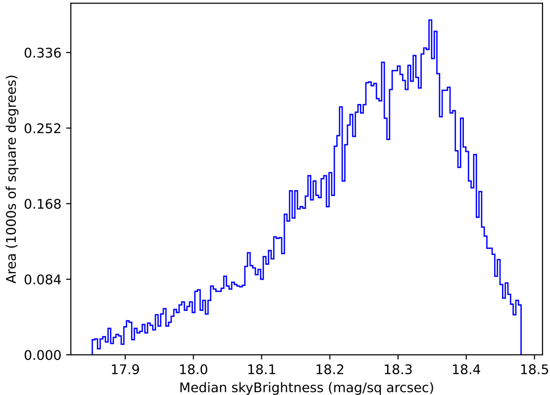
early_ss_template_fpextra2.0_v3.4_10yrs Yr 1 y band: Median skyBrightness
